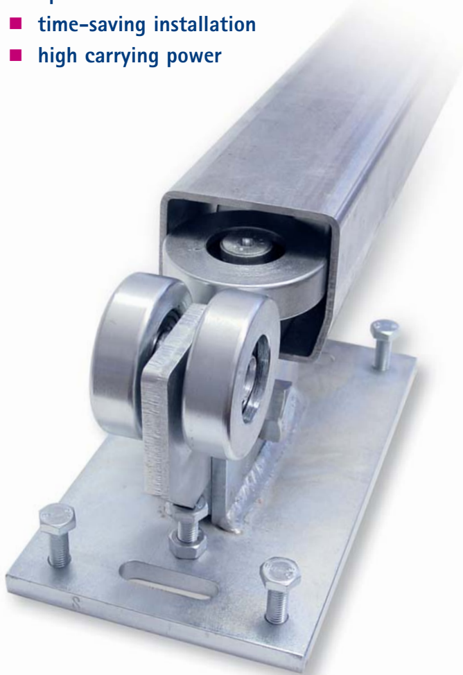
Rollenbock Rollco® LWS 110
